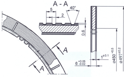
Fig. 1. Geometric data of a sintered friction disc
