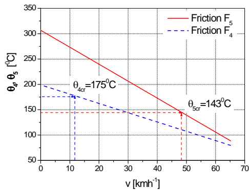
Fig. 10. The limiting braking conditions at maximum speeds
