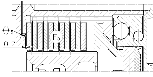
Fig. 4. Position of the temperature sensor
