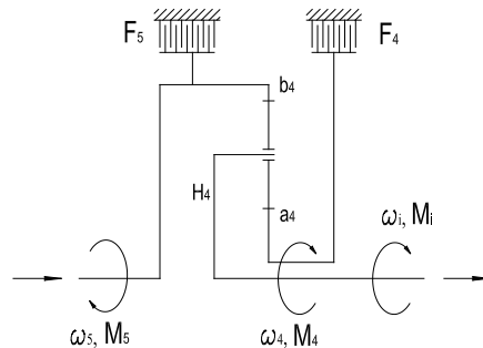
Fig. 3. Positions of the examined brakes in the scheme of the planetary gearbox
