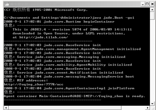
Fig. 5. Startup interface of JADE platform
