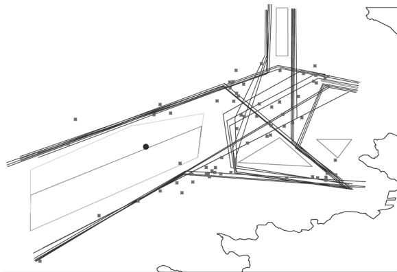
Fig. 10. Simulated places of collisions in scenario 1 during 1600×5 years period with modified TSS and offshore LNG terminal as an obstruction
