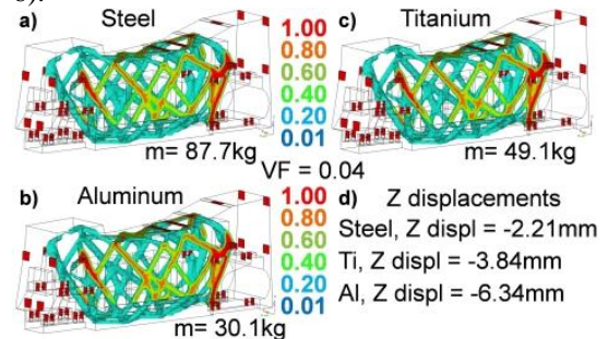
Fig. 11. TO for the vertical bump rear load: a) steel, b) titanium, c) aluminum, d) Z displacements
