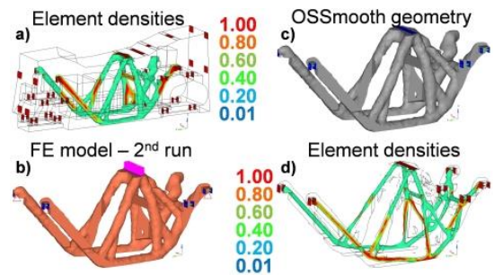
Fig. 12. TO results of the bending: a) 1 st run, b) geometry extraction, c) 2 nd run, d) 2 nd run
