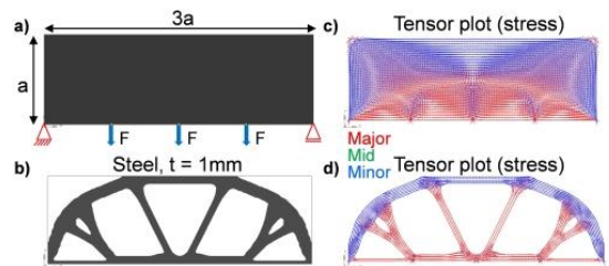
Fig. 5. Generalization of the TO results : a) FE model, b) results for steel, c) original shape, d) optimized shape
