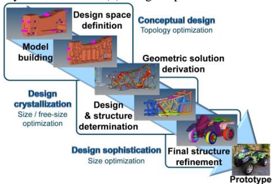
Fig. 2. ICDDP – steps and main development phases
