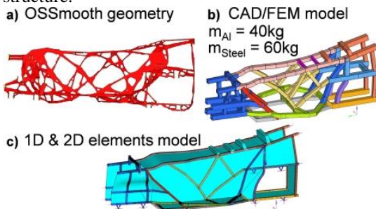
Fig. 17. Geometric solution derivation: a) bionic geometry, b) CAD / FEM interpretation, c) FE model for design crystallization
