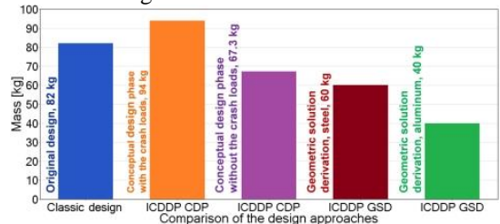
Fig. 18. Comparison of the design approaches: ICDDP CDP – conceptual design phase of the ICDDP; ICDDP GSD – geometric solution derivation step of the ICDDP
