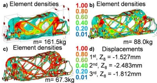
Fig. 16. TO for the influence of crash loads: a) 1 st run, b) 2 nd run, c) 3 rd run, d) Z displacements
