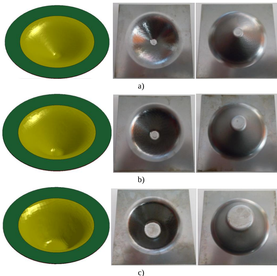
Fig. 10. Experimental parts; a) FEM model and manufactured part for \phi = 40^\circ , H=35\text{mm} , \Delta z=0.5\text{mm} configuration; b) FEM model and manufactured part for \phi = 50^\circ , H=45\text{mm} , \Delta z=0.5\text{mm} configuration; c) FEM model and manufactured part for \phi = 60^\circ , H=50\text{mm} , \Delta z=0.5\text{mm} configuration
