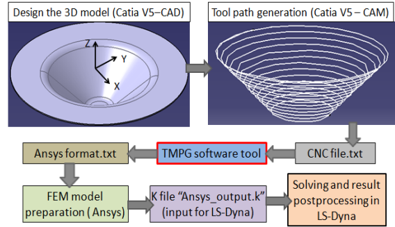
Fig. 7. Main steps for the implementation of FEM simulation
