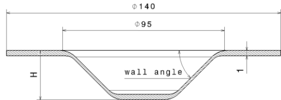
Fig. 6. Experimental frustum of cone
