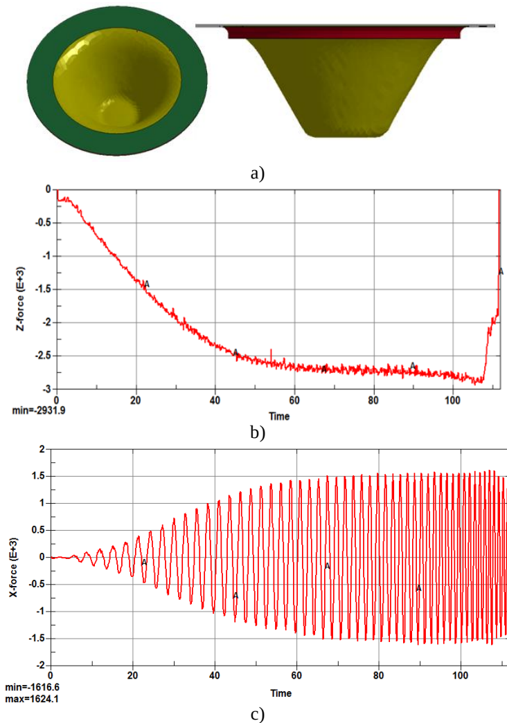
Fig. 8. Obtained results for \phi = 60^\circ , H = 50\text{mm} and \Delta z = 1\text{mm} part configuration; a) resulted FEM model; b) axial force plot; c) radial force plot
