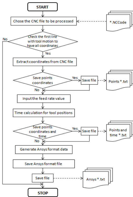
Fig. 2. Software tool block diagram
