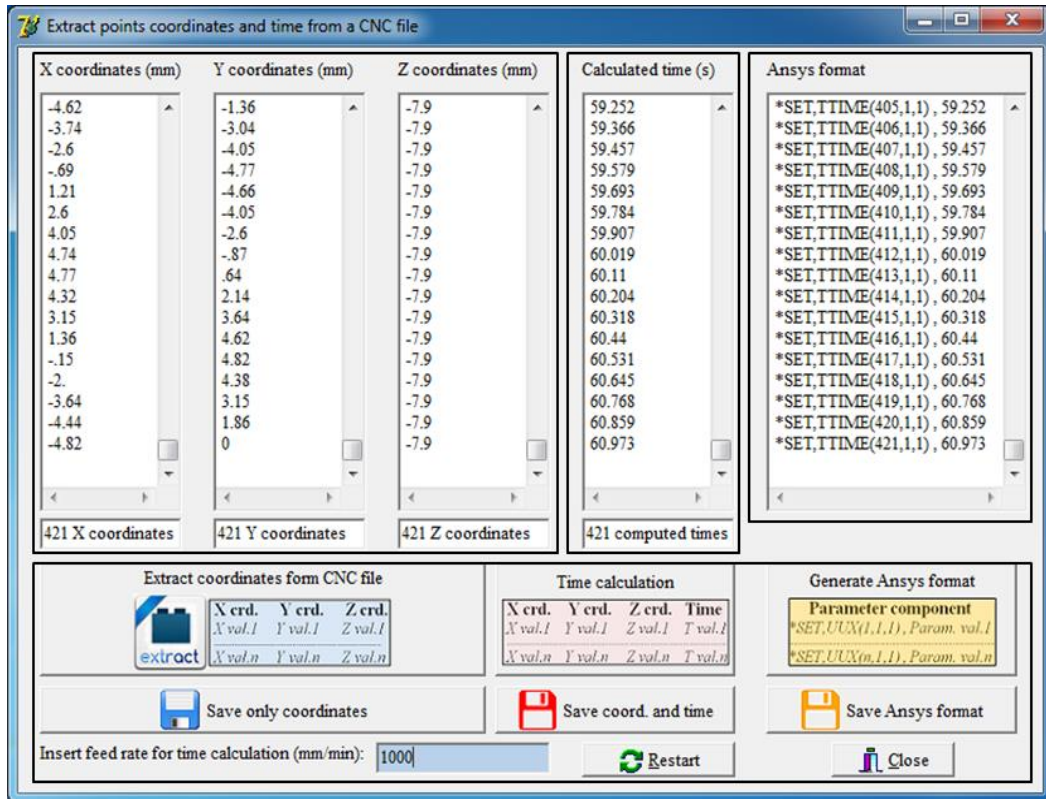
Fig. 3. TMPG software tool interface
