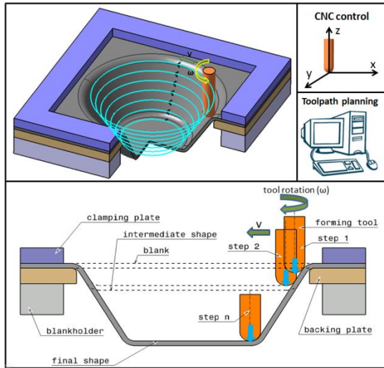
Fig. 1. ISF working principle [2, 3]
