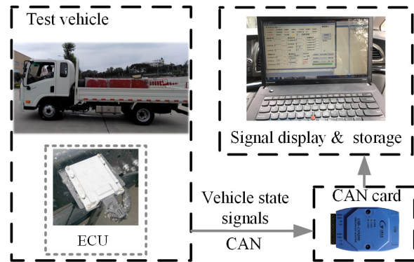
Fig. 13. Experimental setup
