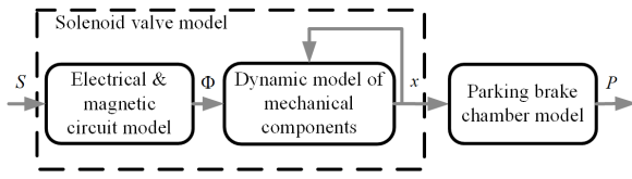
Fig. 5. EPB pneumatic system
