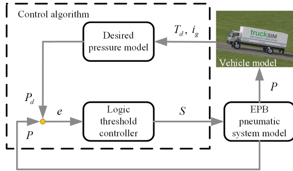
Fig. 3. Block diagram of proposed control system
