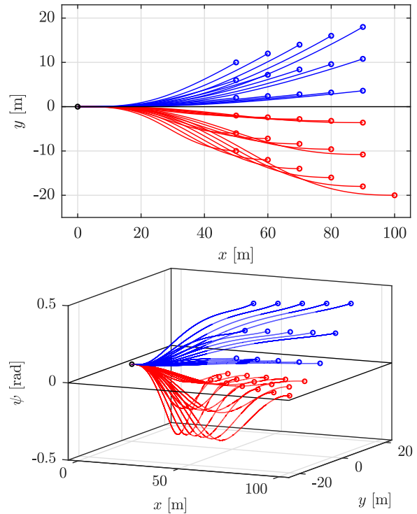
Fig. 5. Sample trajectories
