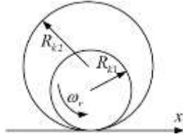
Fig. 2 Finite-length line contact model
