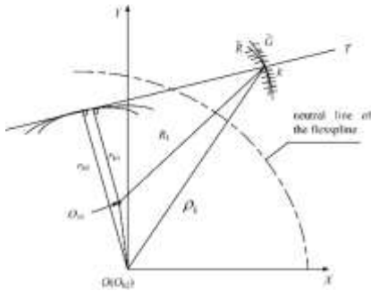
Fig. 3 Schematic diagram of the transmission relationship of the meshing point
