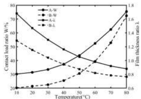
Fig. 10 Effect of oil temperature on lubrication
