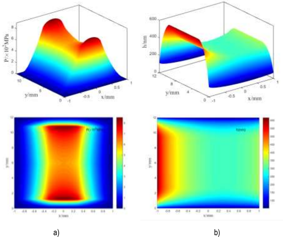
Fig. 8 Numerical solution of pressure and film thickness in the meshing area; (a) pressure distribution, and (b) oil film thickness distribution
