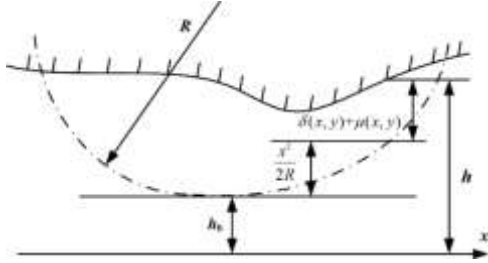
Fig. 7 Schematic diagram of film thickness
