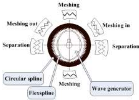
Fig. 1 Schematic diagram of harmonic gear drive
