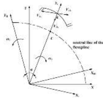
Fig. 4 Schematic diagram of meshing point speed
