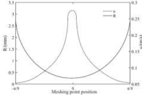
Fig. 5 The variation of comprehensive curvature radius R and entrainment speed u
