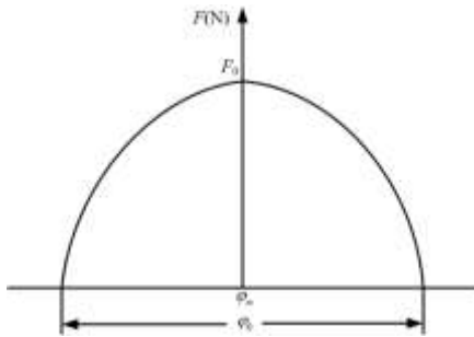
Fig. 6 Simplified curve of load distribution
