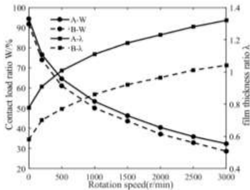
Fig. 9 Effect of rotation speed on lubrication
