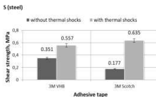
Fig. 6. The shear strength of steel adhesive joints subjected and not subjected to thermal shock testing
