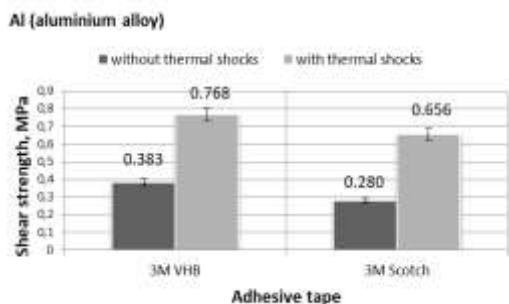
Fig. 7. The shear strength of the aluminium alloy adhesive joints subjected and not subjected to thermal shock testing
