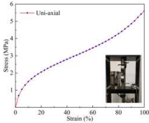
Fig. 2. Stress-strain relationship of PU material
