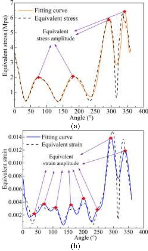
Fig. 7. Fitting curve of equivalent stress and strain of a mesh element; a) Equivalent stress; b) Equivalent strain
