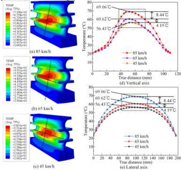
Fig. 9. Steady-state temperature field distribution under different driving speeds
