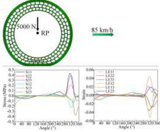
Fig. 5. Stress and strain curve of a mesh element
