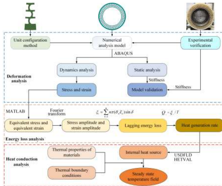
Fig. 4. Flow chart of thermal mechanical coupling characteristics analysis
