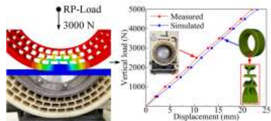
Fig. 3. Comparison of vertical stiffness curves of simulation and test
