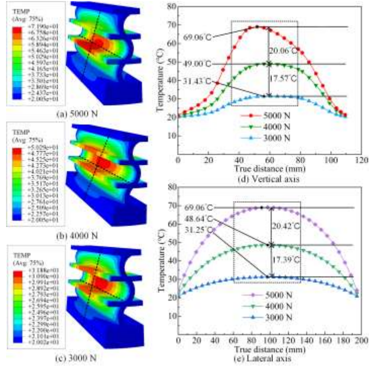
Fig. 10. Steady-state temperature field distribution under different loads
