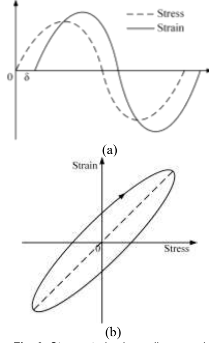
Fig. 6. Stress-strain phase diagram; a) Stress-strain phase relationship; and b) lagging loop
