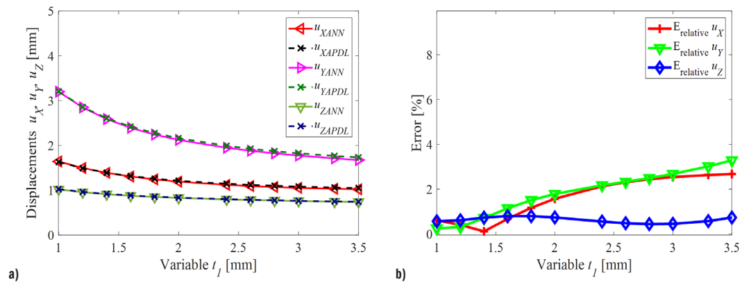
Fig. 12. Comparison of ANN-predicted and APDL-computed displacement components versus parameter t_l ; a) displacement; b) relative error
