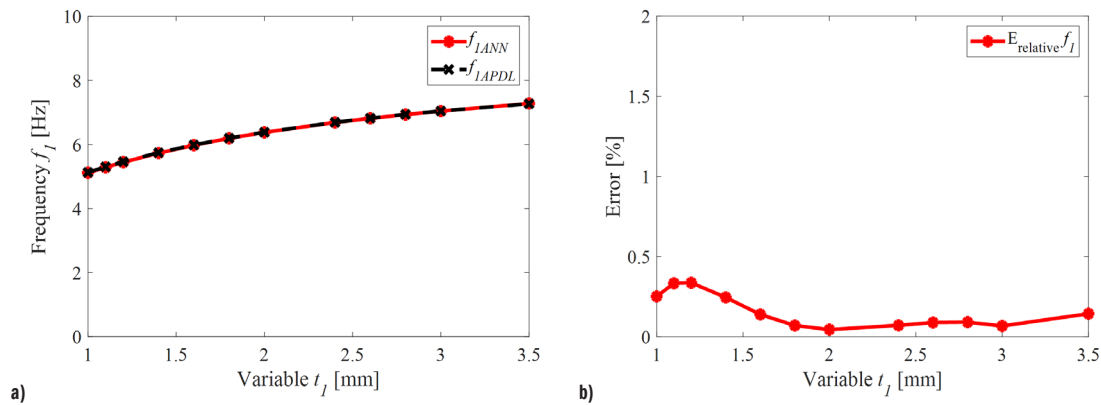
Fig. 13. Comparison of ANN-predicted and Ansys APDL-simulated first natural frequency and the corresponding relative error versus t_l ; a) first natural frequency; b) relative error
