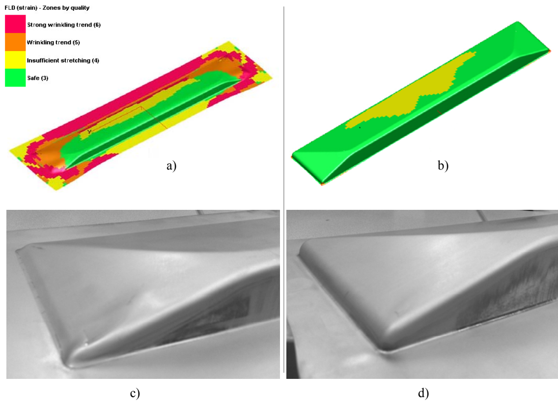
Fig. 11. Wrinkling trend a) step 4 (FEM), b) step 10 (FEM), c) early step (experiment) and d) final draw (experiment)
