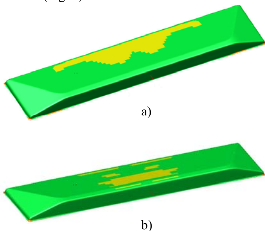
Fig. 7. Good workpieces made by segmented holding system a) with segmented holding forces 306kN b) with segmented holding forces 734kN
