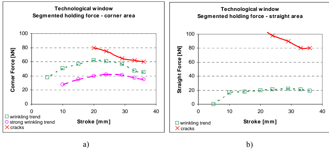
Fig. 10. Technological window for; a) corner areas and b) straight areas
