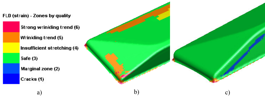
Fig. 4. Critical areas of the workpiece; a) colour scheme, b) wrinkling trend and c) cracks
