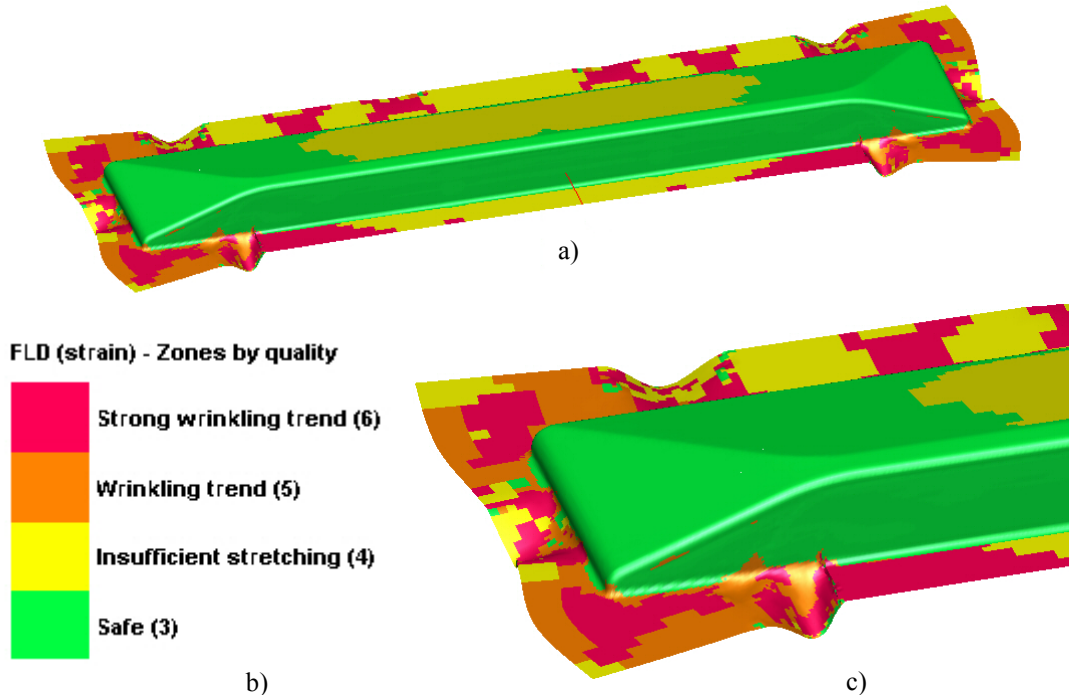
Fig. 6. Flange wrinkling; a) whole model, b) colour scheme, c) detailed view
