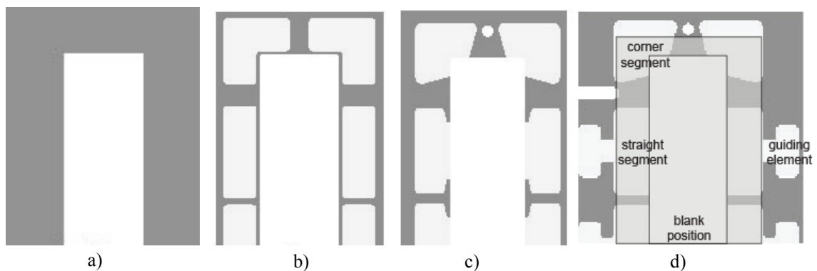
Fig. 5. Conventional blankholder (a) and three versions of segmented blankholder
