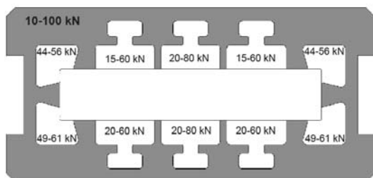
Fig. 8. Ranges for holding forces for each segment
