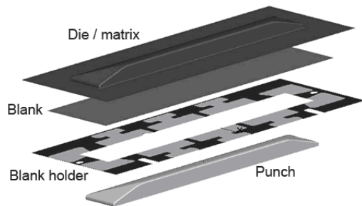
Fig. 3. Computer model
