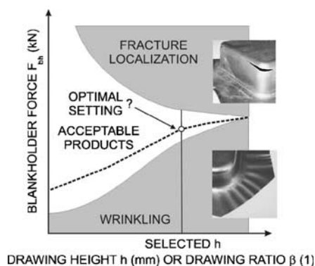
Fig. 1. Technological window [1]
