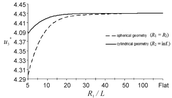
Fig. 11. Variation of central normalized deflection u_3^* at varying shallowness ratios for spherical and cylindrical shells
