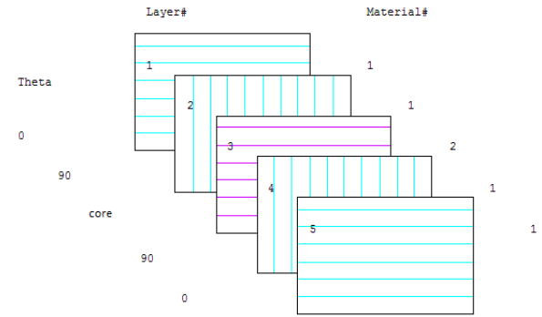
Fig. 6. Layered element model for a 0^\circ/90^\circ/\text{core}/90^\circ/0^\circ laminate
