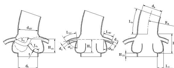
Fig. 2. Important geometric parameters of computational domain
