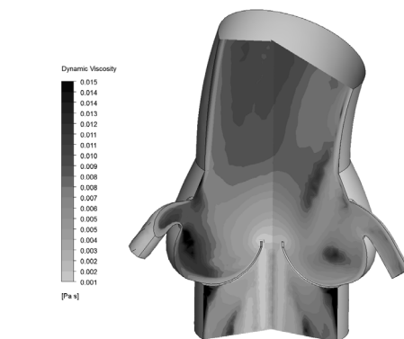
Fig. 13. Dynamic viscosity field for regurgitated aortic valve (0.35 s)
