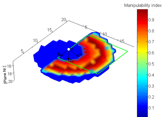
Fig. 6. 3D-plot of manipulability indices in an open workspace at slice plane 15 of 21 (the white point indicates the origin coordinates of the mechanism and the green frame indicates limited space)
