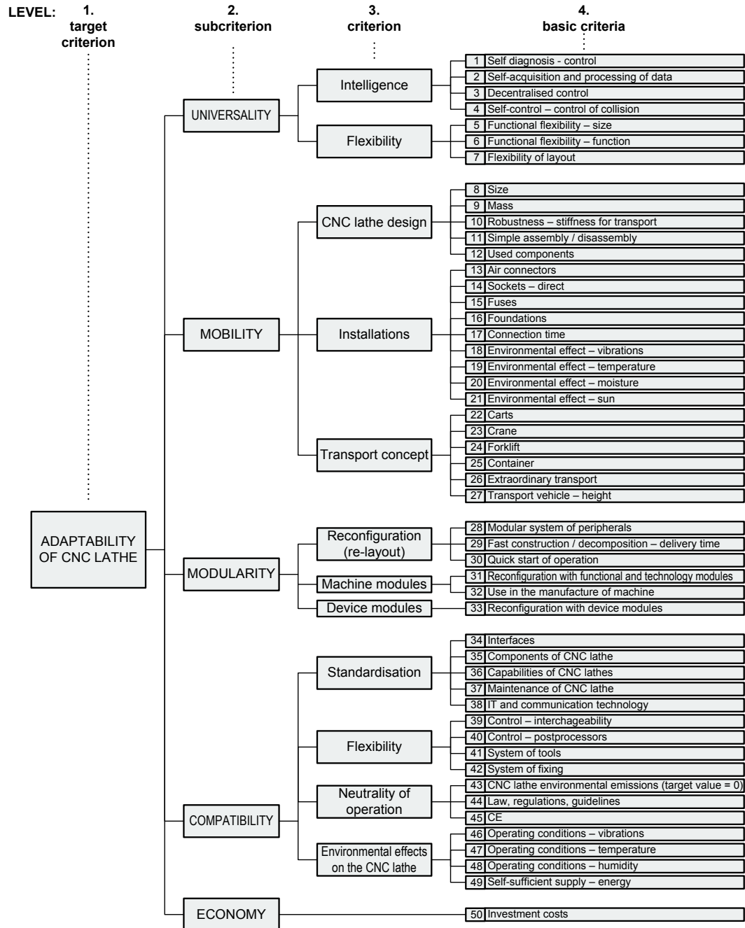
Fig. 4. The criteria for assessing the adaptability of a CNC lathe
