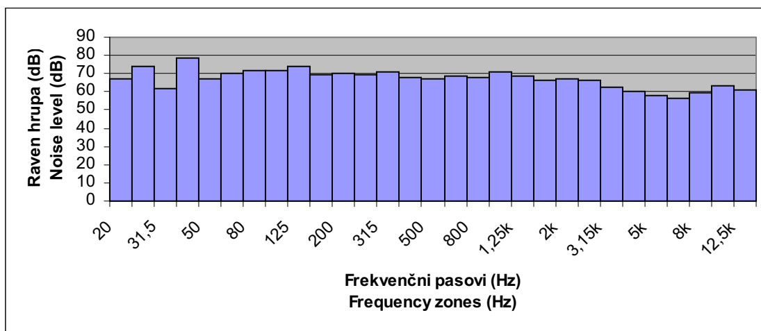
Sl. 1. DM 4, opravi 1 (grobo frezanje) Fig. 1. WP 4, operation 1 (coarse milling)
