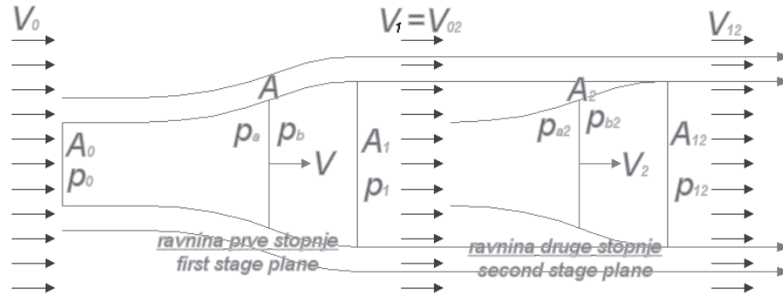
Sl. 2. Model dvostopenjske vetrne turbine Fig. 2. Double-stage wind-turbine model
