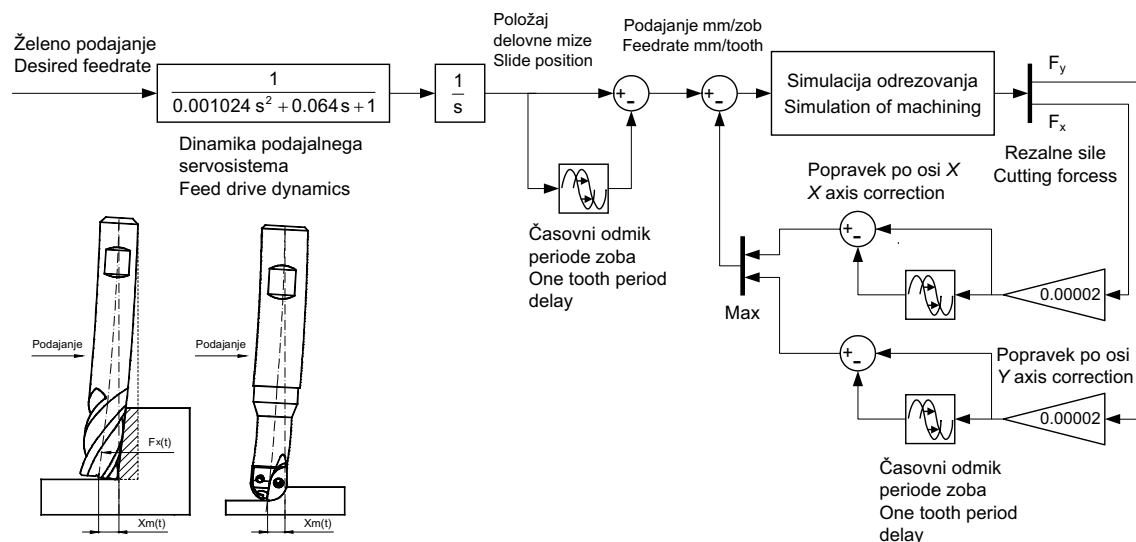
Sl. 3. Simulator RNK frezanja
