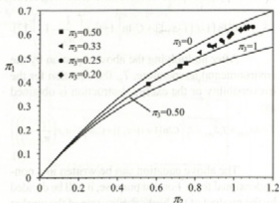
Fig. 3. The positions of the measured operation points for a counter-flow heat exchanger
