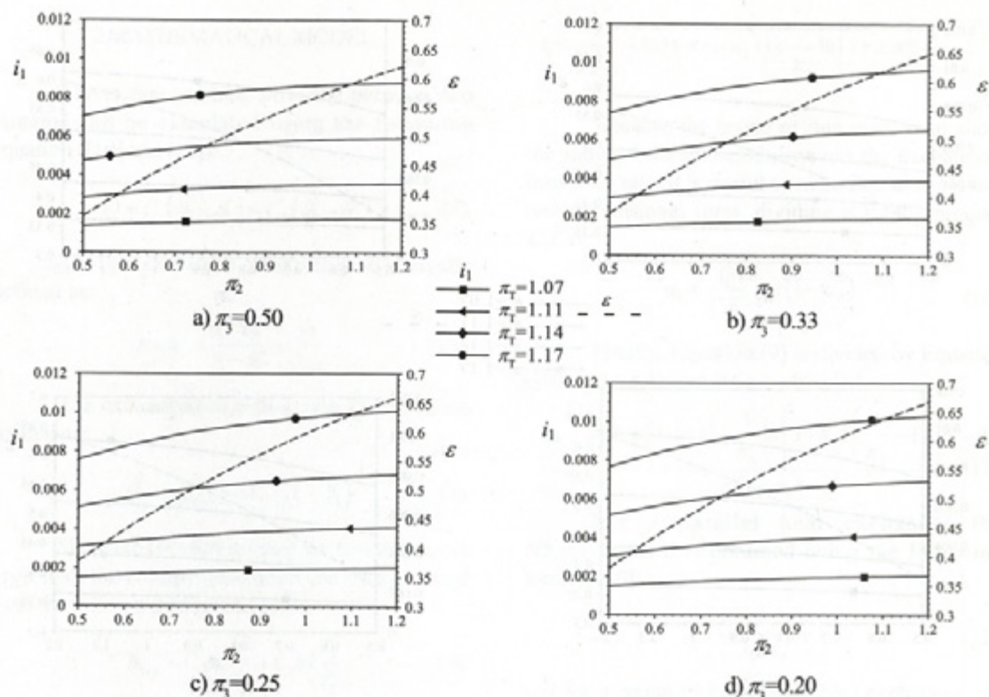
Fig.6. Non-dimensional irreversibility i_1 and effectiveness \varepsilon as a function of \pi_2 and the parametric curves \pi_1 for a) \pi_3=0.50 , b) \pi_3=0.33 , c) \pi_3=0.25 d) \pi_3=0.20 for a counter-flow heat exchanger
