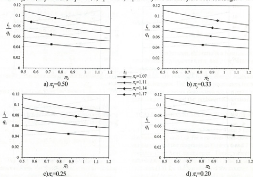
Fig. 7. Relative non-dimensional irreversibility i_1/q_1 as a function of \pi_2 and the parametric curves \pi_1 for a) \pi_3=0.50 , b) \pi_3=0.33 , c) \pi_3=0.25 , d) \pi_3=0.20 for a counter-flow heat exchanger
