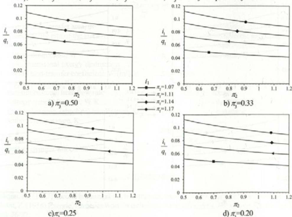
Fig. 5. Relative non-dimensional irreversibility i_1/q_1 as a function of \pi_2 and the parametric curves \pi_r for a) \pi_3 = 0.50 , b) \pi_3 = 0.33 , c) \pi_3 = 0.25 , d) \pi_3 = 0.20 for a parallel-flow heat exchanger
