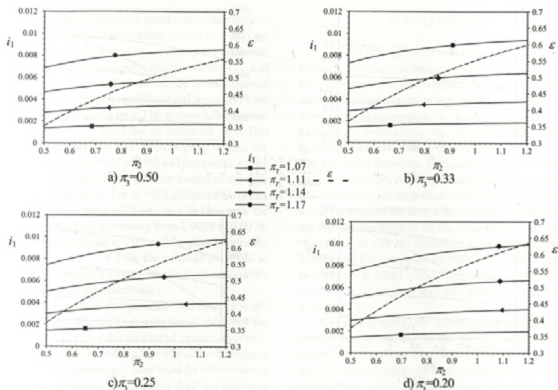
Fig. 4. The non-dimensional irreversibility i_1 and the effectiveness \varepsilon as a function of \pi_2 and the parametric curves \pi_r for a) \pi_3 = 0.50 , b) \pi_3 = 0.33 , c) \pi_3 = 0.25 and d) \pi_3 = 0.20 for a parallel flow heat exchanger
