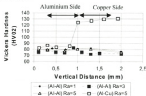
Fig. 17. Hardness variations along the vertical direction
