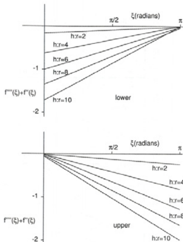
Fig. 9. Graphs of f'''(\xi) + f''(\xi) for various height:radius ratios and back angles \theta_0 with \beta = 10^\circ and \beta = 90^\circ
