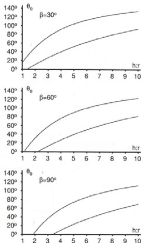
Fig. 7. Upper and lower bounds of back angle \theta_0 for front angle \theta_1 = 30^\circ and various opening angles \beta
