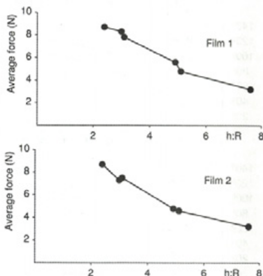
Fig. 10. Forces required to pull films over shoulders
