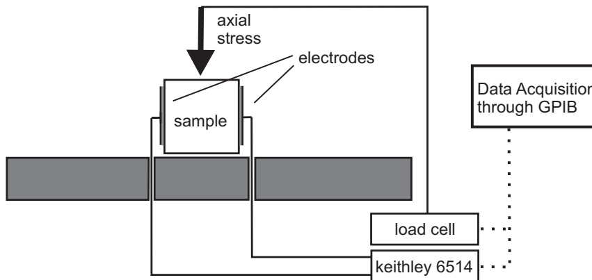
Fig. 2. Schematic diagram of the experimental setup
