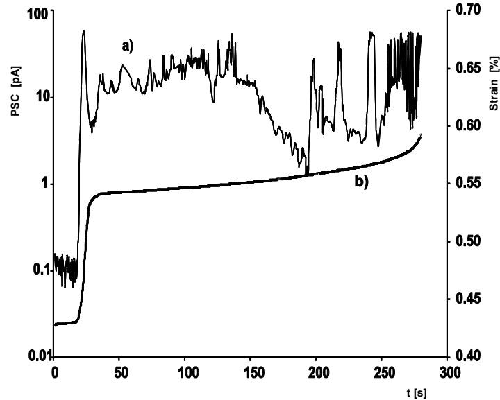
Fig. 5. a) The temporal variation of the PSC during the last stress step and b) the corresponding temporal recording of the deformation
