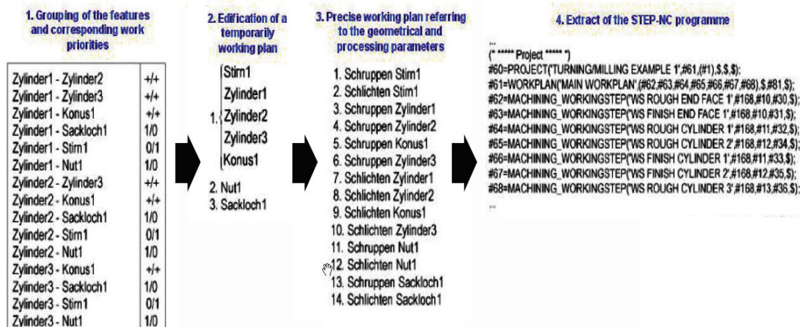
Fig. 4. Process planning in the STEPurn [4]
