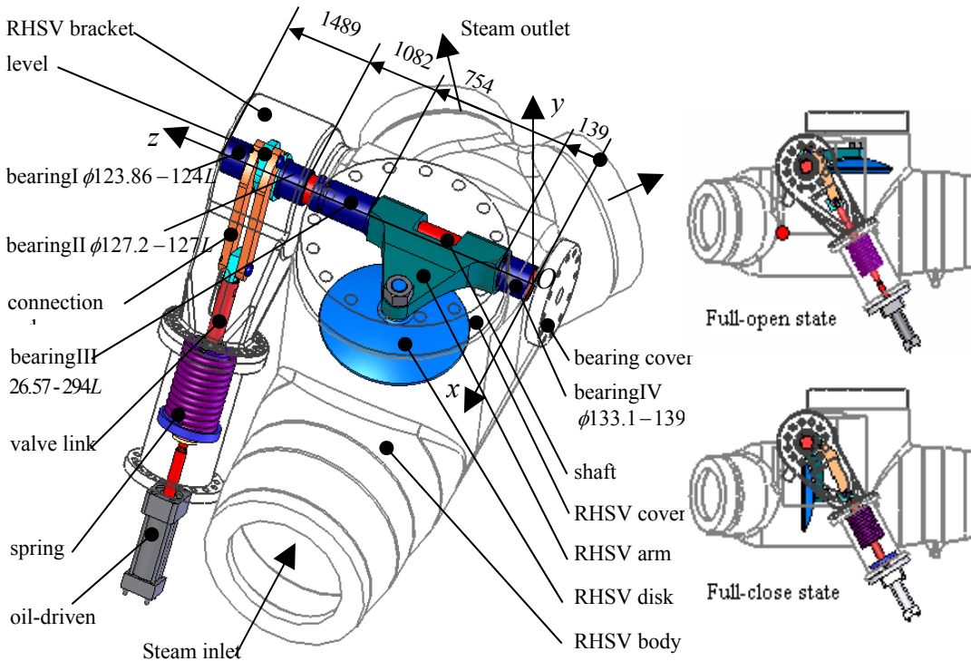
Fig. 1. Three dimensional structure of the RHSV mechanism
