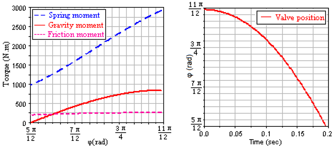
(a) Driving and friction moment when closing valve (b) Dynamic performance when closing valve
