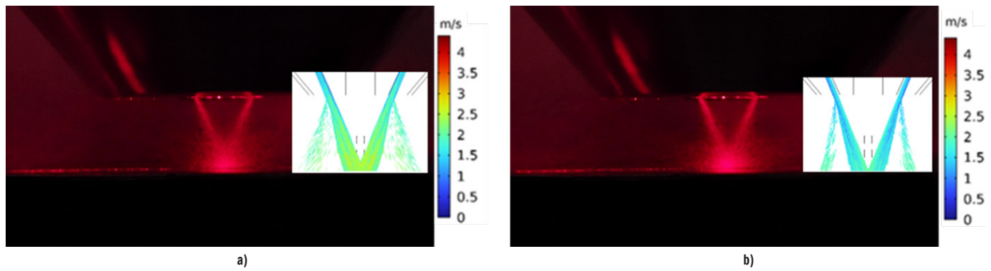
Fig. 17. Narrow Nozzle experimental particle flow visualization (a)NN4, (b)NN3
