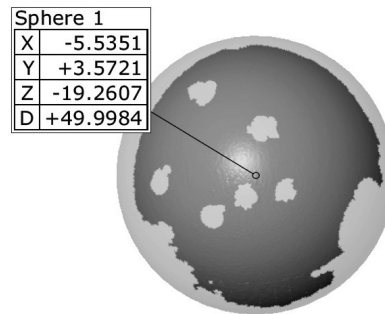
Fig. 20. Sphere primitive definition from scanned data
