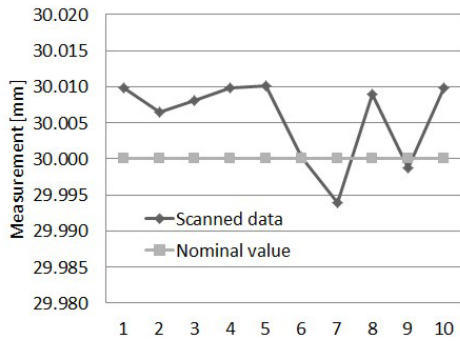
Fig. 15. Results of the 30 mm gauge block scanning
