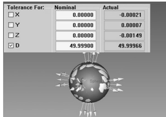
Fig. 19. CMM sphere inspection
