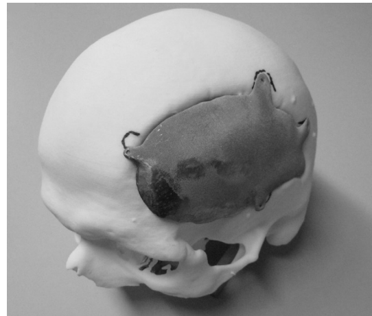
Fig. 2. Cranial implant and skull model
