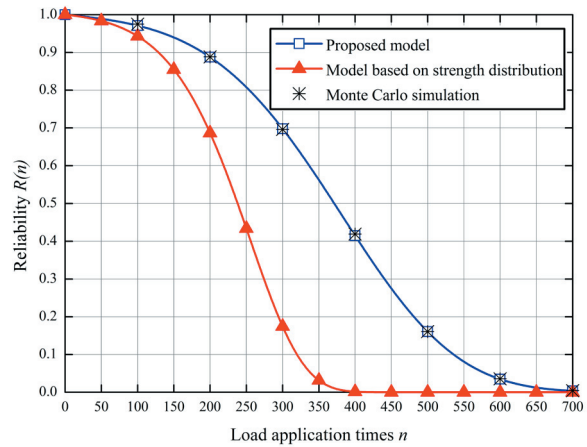
Fig. 6. Comparison between proposed method and Monte Carlo simulation
