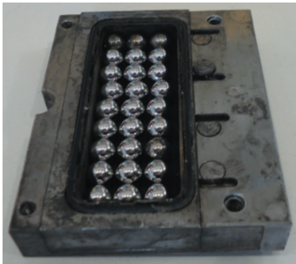
Fig. 6. Mould slot filled with bearing balls
