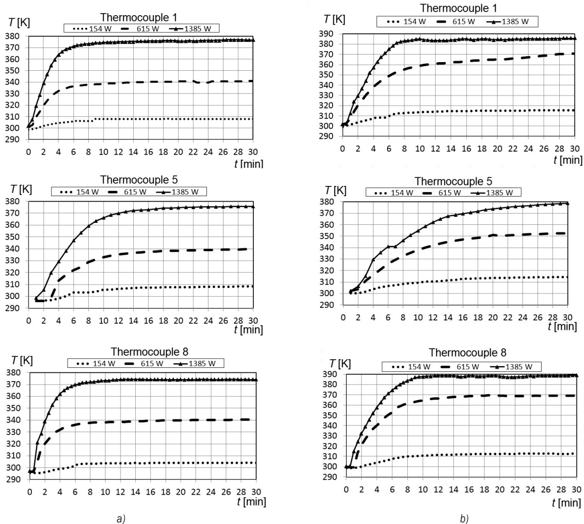
Fig. 5. Temperature behavior measured by thermocouples t_1 , t_5 and t_8 , for three heating conditions in the evaporator (154, 615, 1,385 W) versus time; a) for a cooling water flow of 16.67 \text{ cm}^3/\text{s} and b) for a cooling water flow of 4.17 \text{ cm}^3/\text{s}
