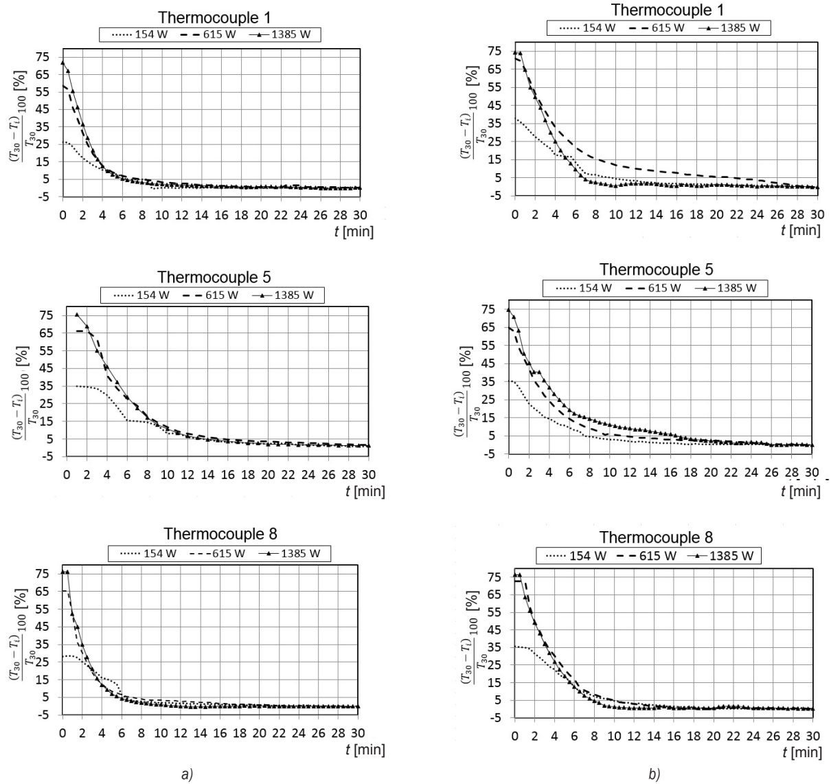
Fig. 6. Percent variation of temperatures t_1 , t_5 and t_8 for three heat flow levels; a) for a cooling water flow of 16.67 \text{ cm}^3/\text{s} and b) for 4.17 \text{ cm}^3/\text{s}
