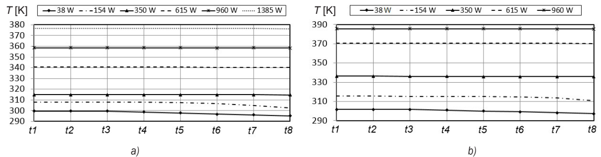
Fig. 7. Temperature values measured for the different thermocouples t_1 to t_8 for 38, 154, 350, 615, 960 and 1385 W of heat flow levels supplied, with cooling water flow of a) 16.67 \text{ cm}^3/\text{s} and b) 4.17 \text{ cm}^3/\text{s} , 30 minutes after the experiment start
