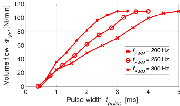
Fig. 5. Comparison of test results for pressure difference \Delta P = 6 bar and different PWM frequencies
