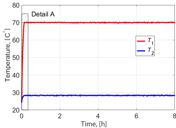
Fig. 13. Change of valve temperature T_1 and T_2
