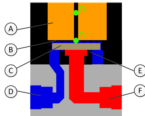
Fig. 4. Schematics of the fast switching valve internal components
