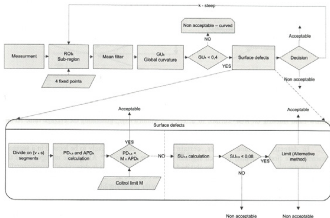
Fig. 5. The flowchart for detection of surface defects
