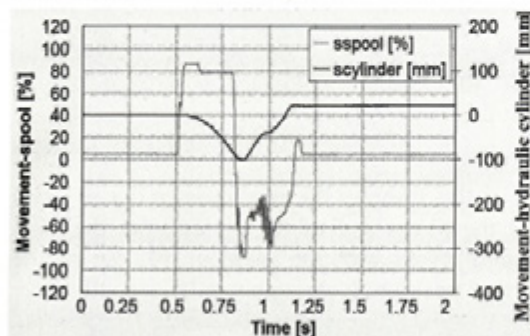
Fig. 9. Movement of the spool and the piston rod of the cylinder with the mass during the loading cycle in the water part of PCH
