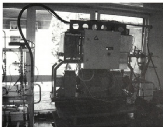
Fig. 3. Oil power-control part of the test rig
