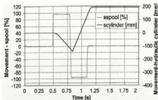
Fig. 8. Movement of the spool and the piston rod of the cylinder with the mass during the loading cycle in the oil part of PCH
