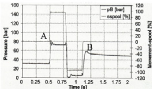
Fig. 10. Movement of the spool and the pressure changes during the experiment with mass - cycle in the oil part of PCH
