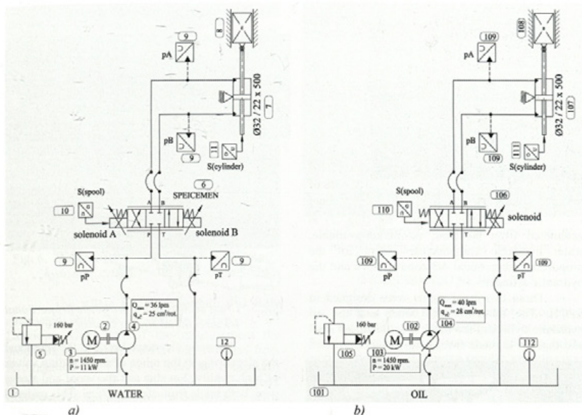
Fig. 1. Hydraulic circuits of the test rig
