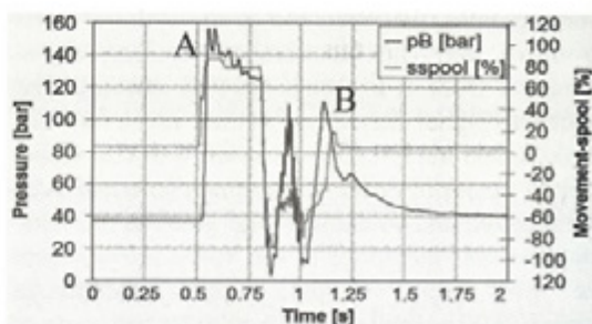
Fig. 11. Movement of the spool and the pressure changes during the experiment with the mass - cycle in the water PCH
