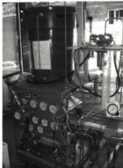
Fig. 2. Water power-control part of the test rig
