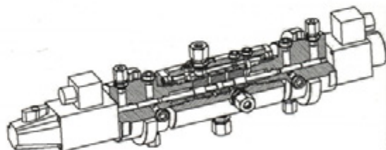
Fig. 5. Cross section of the prototype proportional 4/3 directional sliding control valve
