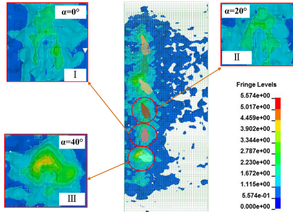
Fig. 11. Stress distribution on coal when cutting by conical picks with different angles
