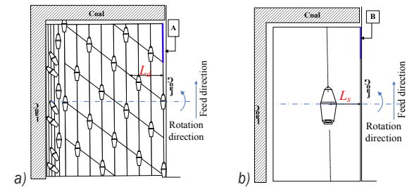
Fig. 3. Simulation model: a) drum model, b) single pick model
