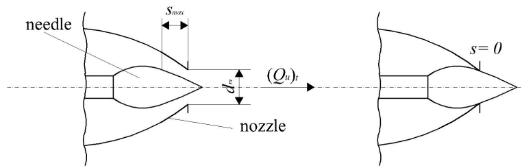
Fig. 1. Pelton turbine distributor (needle valve)
